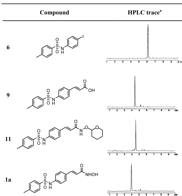
Fig. 1 Purity profile for the flow-through synthesis of hydroxamic acid 1a .
