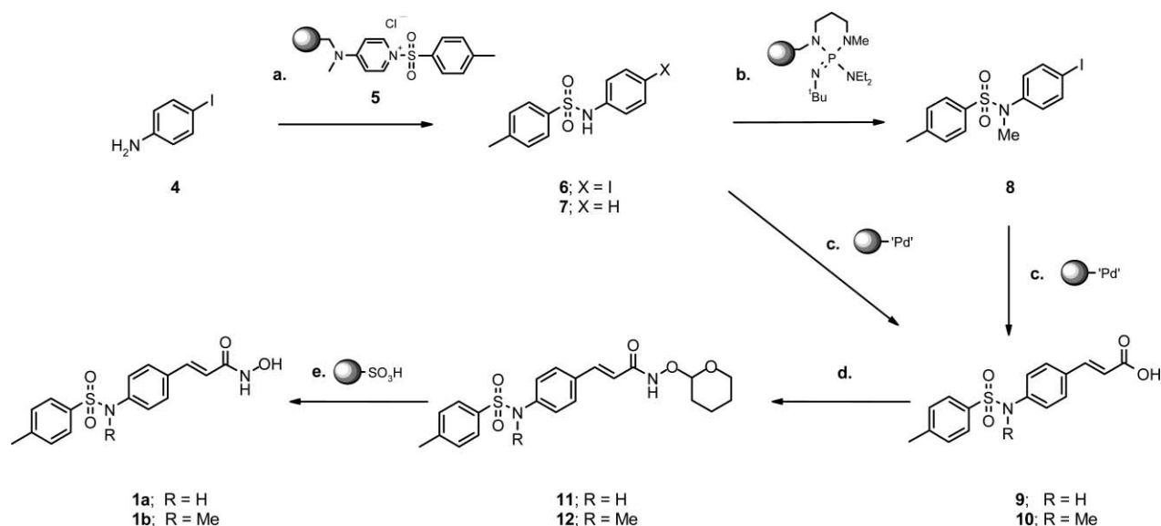
Scheme 1 Reagents and conditions: a) (i). DMF, 50 °C, 1 h, \times 2 ; (ii). SCX SPE purification; b) MeI, DMF, rt, 18 h; c) acrylic acid, triethylamine, DMF, 90 °C, 18 h; d) (i). 1-(3-dimethylaminopropyl)-3-ethylcarbodiimide hydrochloride, 1-hydroxybenzotriazole, DMF, rt, 20 min; (ii). hydroxylamine-OTHP, 50 °C, 18 h; (iii). \text{NH}_2 SPE purification; e) Amberlyst H-15, MeOH, rt, 2 h.
